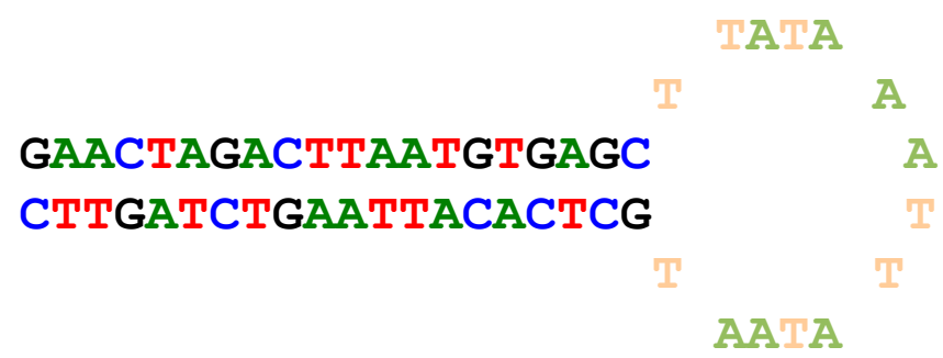
Hairpin structure
